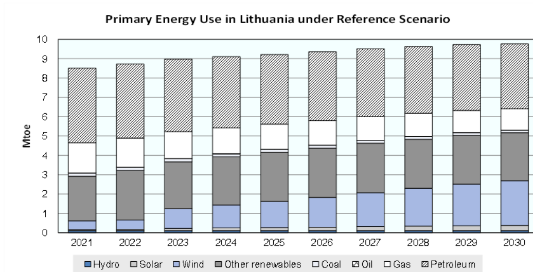
Figure 3.4. Under the reference scenario, primary energy use in Lithuania increases, with particular use of wind energy growing considerably
