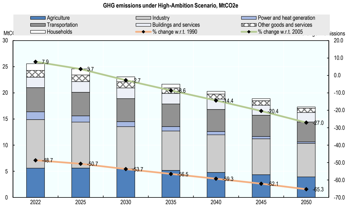
Figure 7.6. Carbon pricing on combustion-based CO 2 emissions alone is not enough for reaching net zero GHG emissions by 2050
